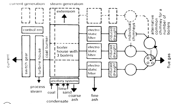
1 Power station schematic diagram
